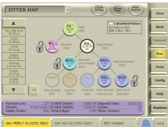
Figure 2.4d. BERT with Jitter Values on a Jitter Map.
