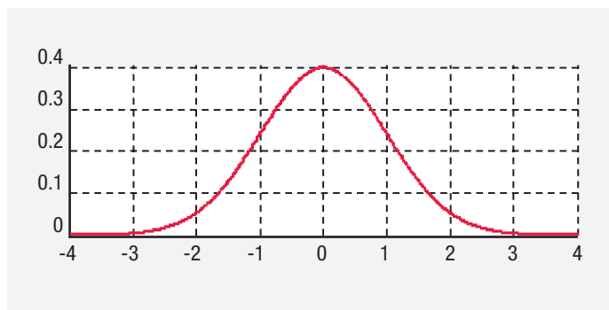
Figure 4.2.1a. Gaussian Distribution.
